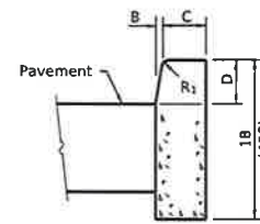
BARRIER CURB
