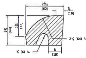
FRONT VANE DETAIL
