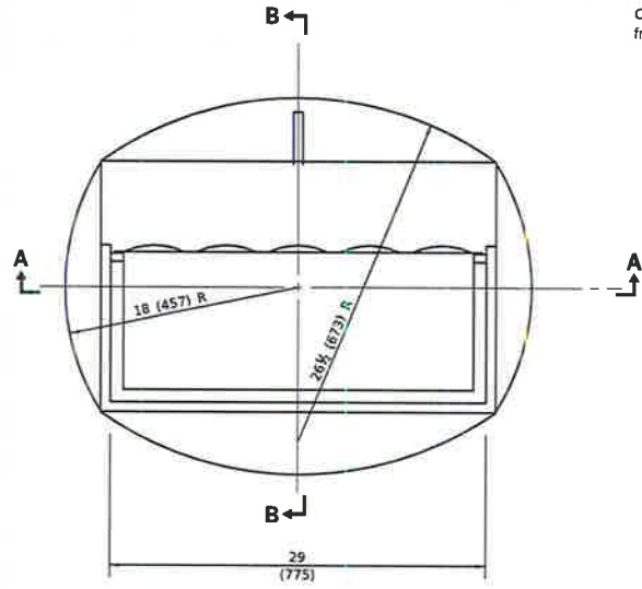
CAST FRAME
