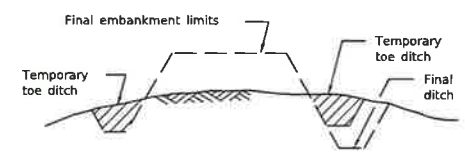
TYPICAL FILL CROSS-SECTION
