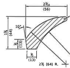
VANE DETAIL
