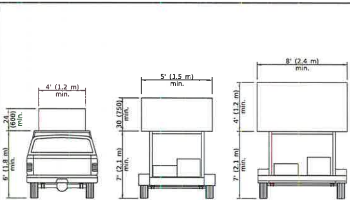
TYPE A ROOF MOUNTED TYPE B ROOF OR TRAILER MOUNTED TYPE C TRAILER MOUNTED
