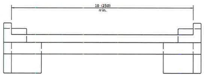
ELEVATION VIEW
