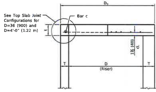
SECTION THRU FLAT SLAB TOP FOR D = 36 (900) AND D = 4'-0" (1.22 m)
