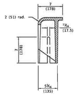
SECTION E-E
