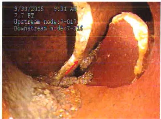
#5: Pipe Defect at 7.7 feet from MH 7-017 (collapsed existing lateral service)
