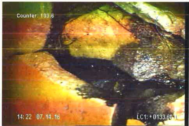
#6: Pipe Defect at 133.6 feet from MH 6-018 (tap break-in, hole void visible and fracture multiple)
