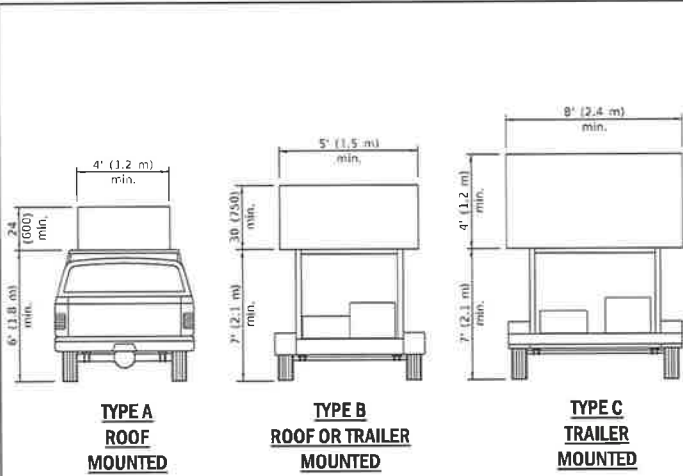
ARROW BOARDS
