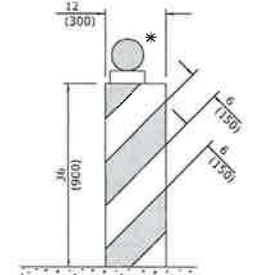
VERTICAL BARRICADE
