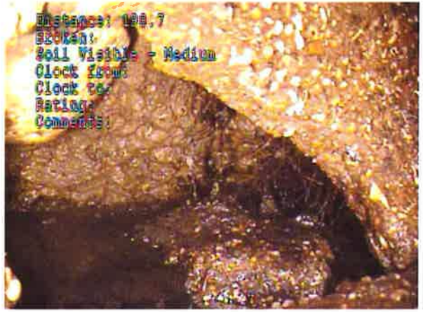
#4: Pipe Defect at 198.7 feet from MH 3-090 (Broken pipe, hole void visible)
