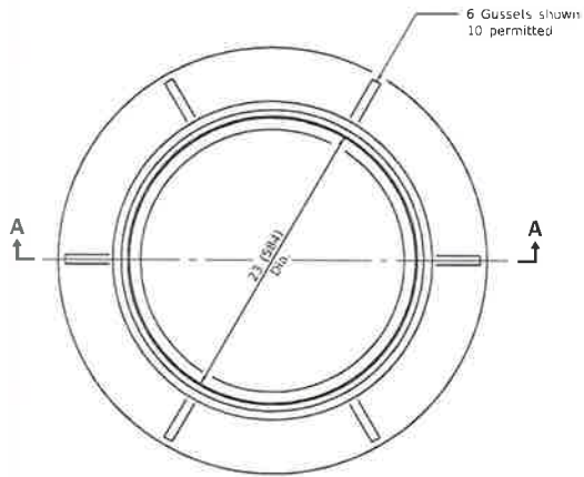
CAST FRAME
