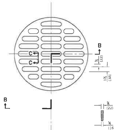
SECTION C-C
